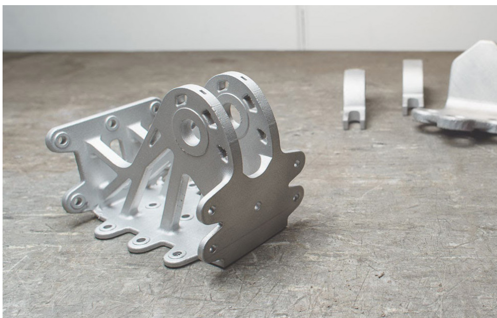
A complex Aluminum bracket produced via Powder Bed Fusion with a design optimized for weight reduction and minimal cost.
