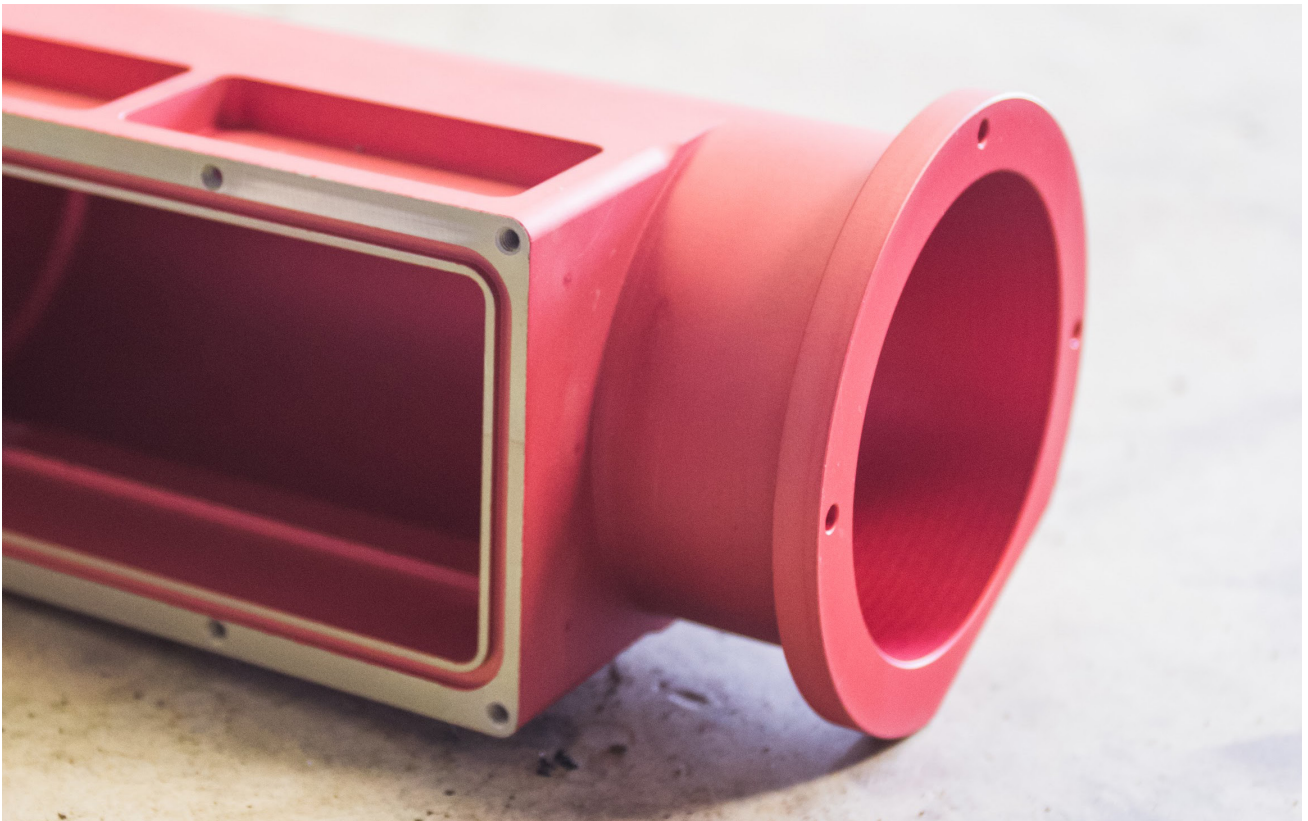
The same CNC aluminum part after red Anodized Type II finish. Chrome plating is added to the visible part, not in red.
