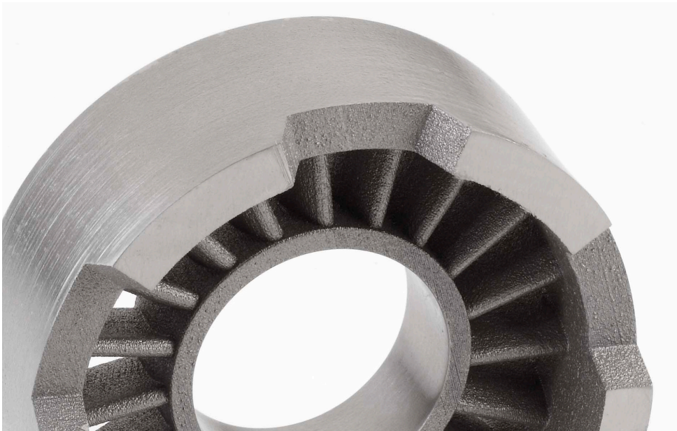
A functional metal part in stainless steel-bronze matrix. Part geometry is less complex than for Powder Bed Fusion as the requirements to save material are less relevant. Image courtesy of ExOne.
