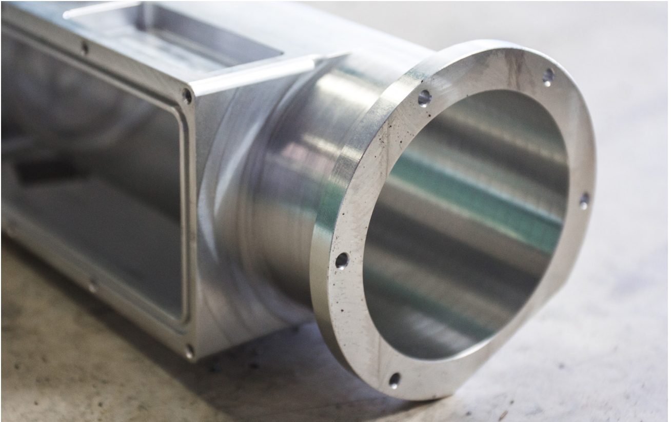
CNC aluminum part with "as machined" finish
